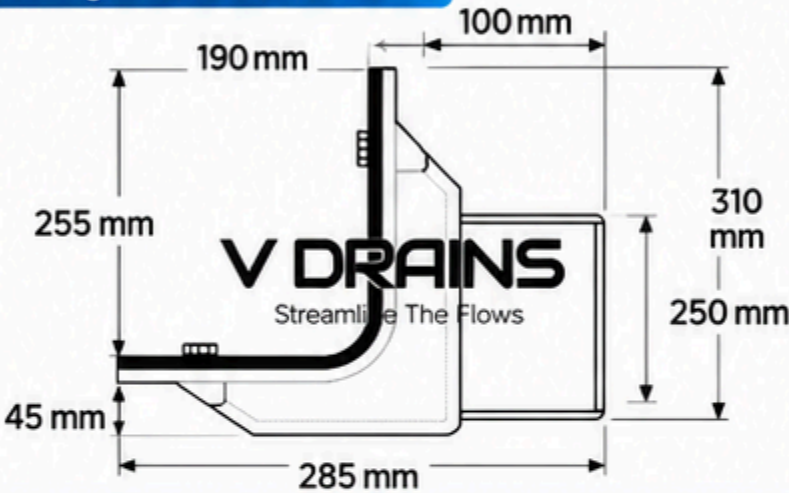
Drawing 1 : Side Section View
