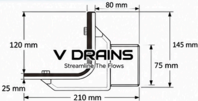
Drawing 1 : Side Section View
