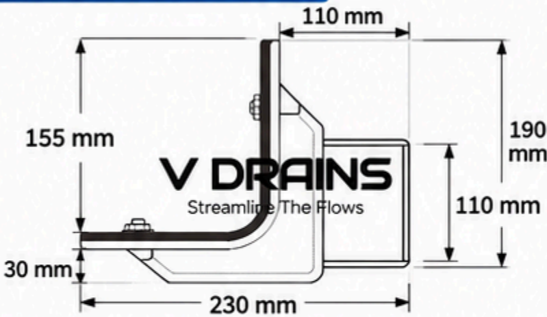
Drawing 1 : Side Section View
